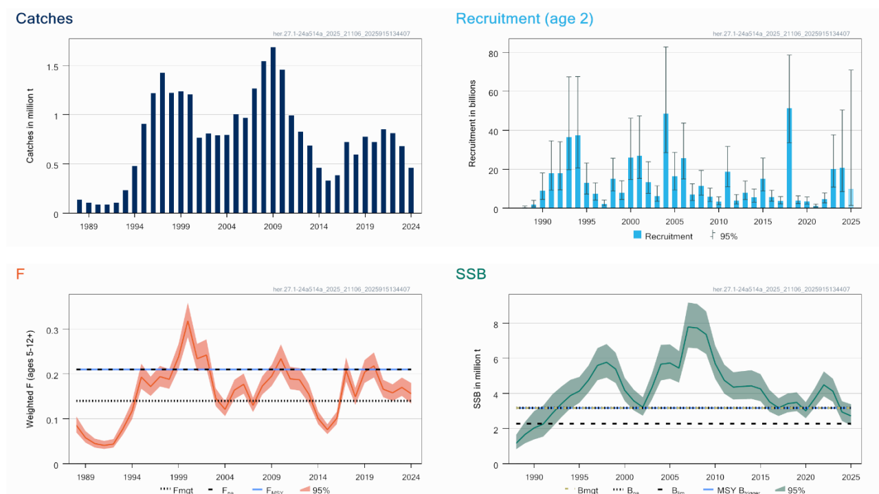
Figure 1 Herring in subareas 1, 2, and 5, and in divisions 4.a and 14.a (Norwegian spring-spawning herring). Summary of the stock assessment. The assumed recruitment value for 2025 is shaded in a lighter colour.
