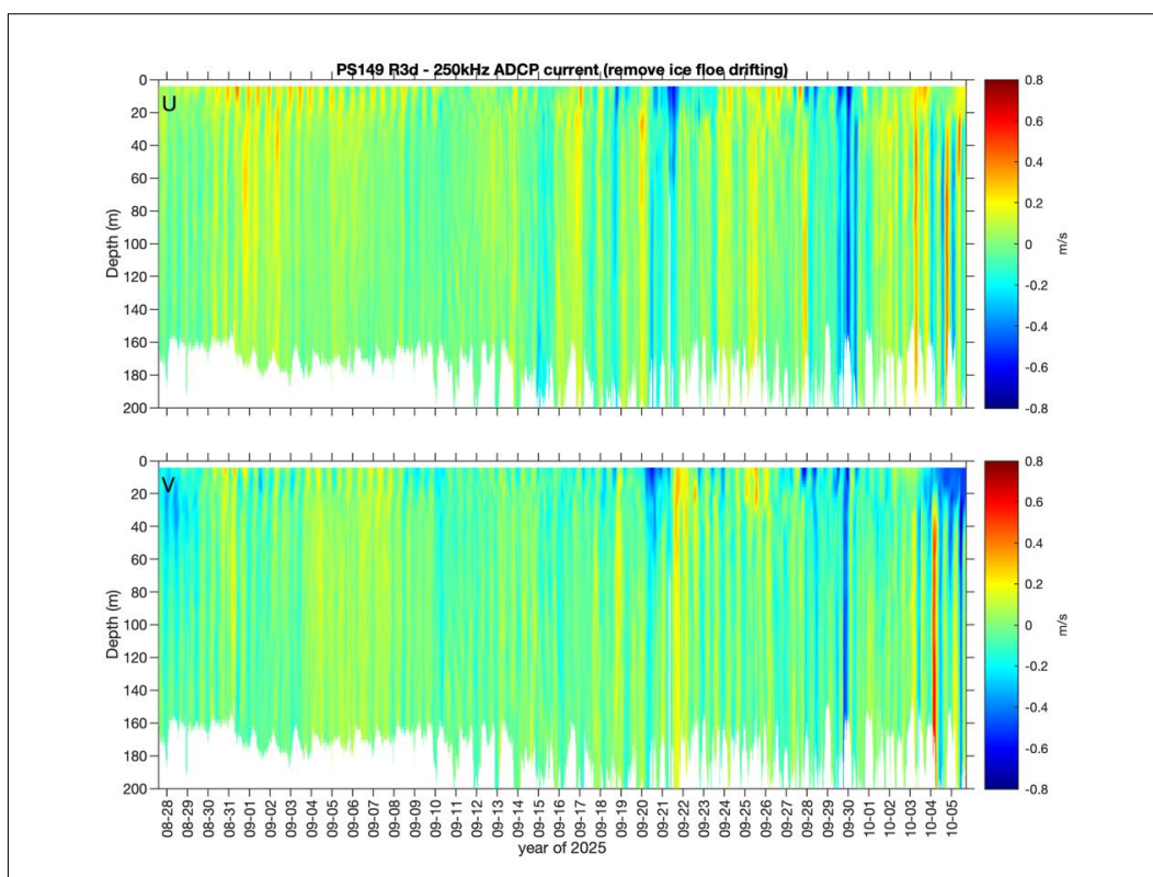
Fig. 2.53: Preliminary plot of the meridional ( u ) and zonal ( v ) components of the ocean current velocities measured by the instrument. Plot by Ke-Hsien Fu
