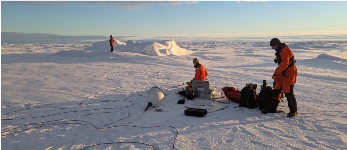
Fig. 2.40: Photo of CTD buoy AWI-SVP5S-0006 (shortcode 2025O34) during preparation, while a fishing-rod CTD is conducted in the ice hole prior to deployment. Photo by Manuel Franco Pire
