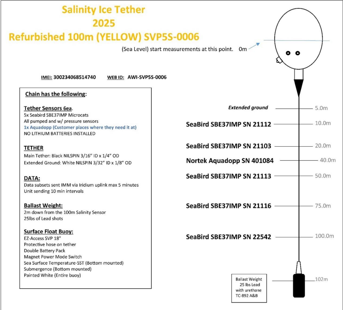
Fig. 2.39: Schematic diagram of CTD buoy AWI-SVP5S-0006 (shortcode 2025O34). Modified after Pacific Gyre by Mario Hoppmann
