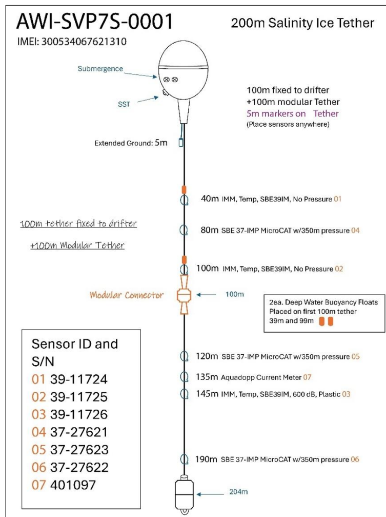
Fig. 2.43: Schematic diagram of SIT-type CTD buoy AWI-SVP7S-0001 (shortname 2025O35). Modified after Pacific Gyre by Mario Hoppmann
