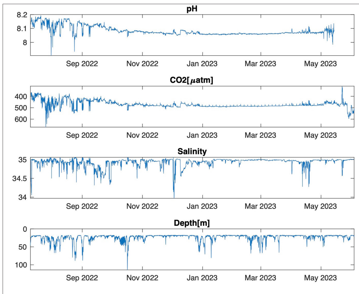
Fig. 5.4: Time series of pH and p\text{CO}_2 , with salinity and depth as reference; data from sensors deployed in mooring F4-S6 recovered on PS136
