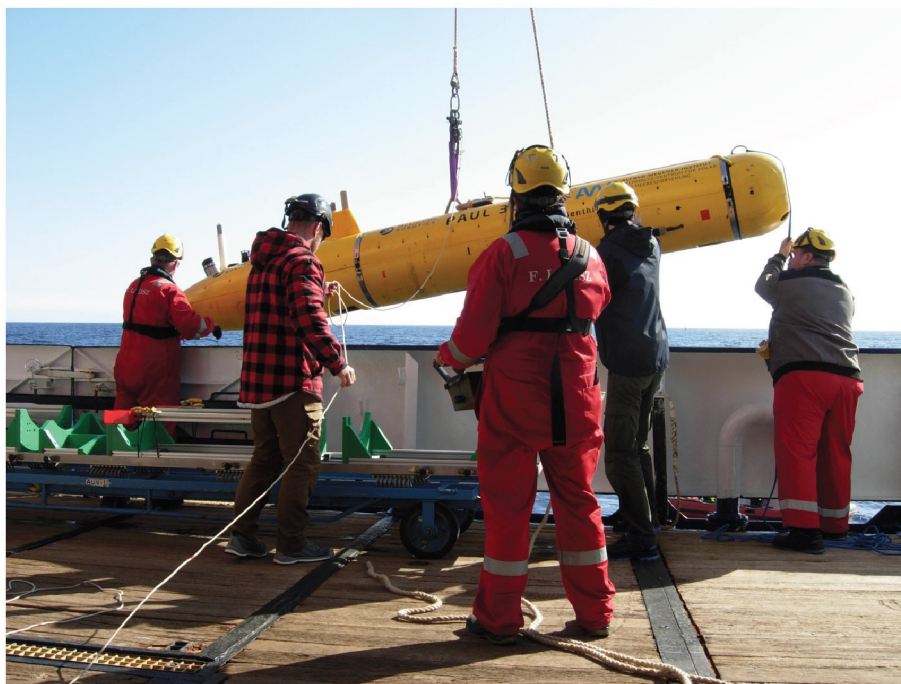
Fig. 3.5: Deployment of the Autonomous Underwater Vehicle "PAUL"
