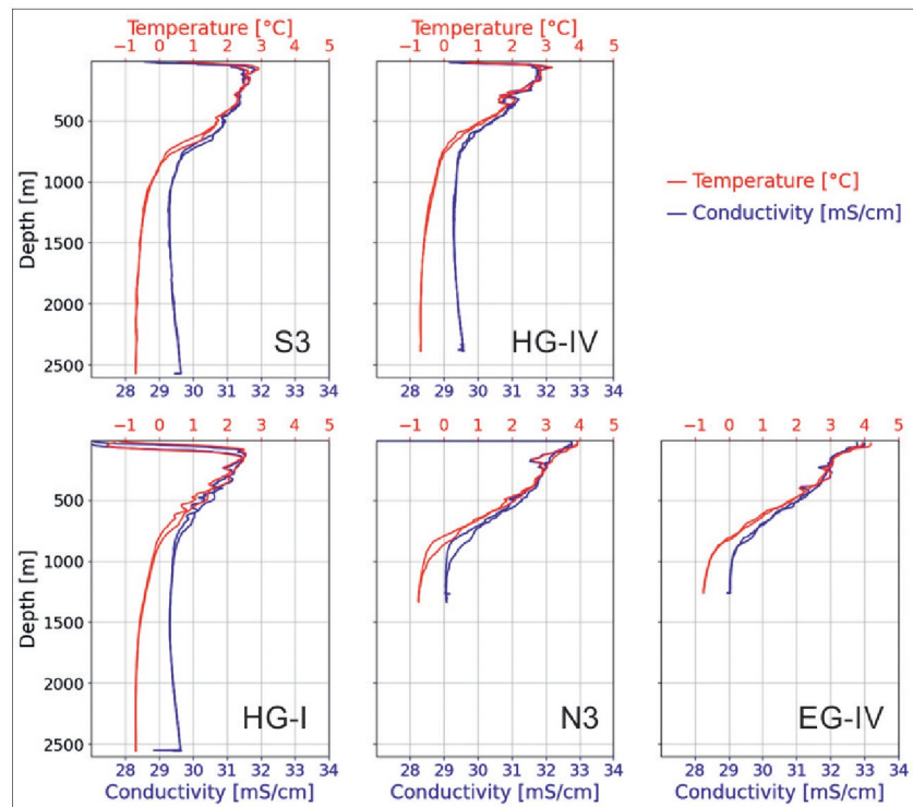
Fig. 3.14: CTD data registered during EBS deployments at five HAUSGARTEN station (no data for HG-IX, because the pressure housing was not depth-rated to 6,000 m water depth)
