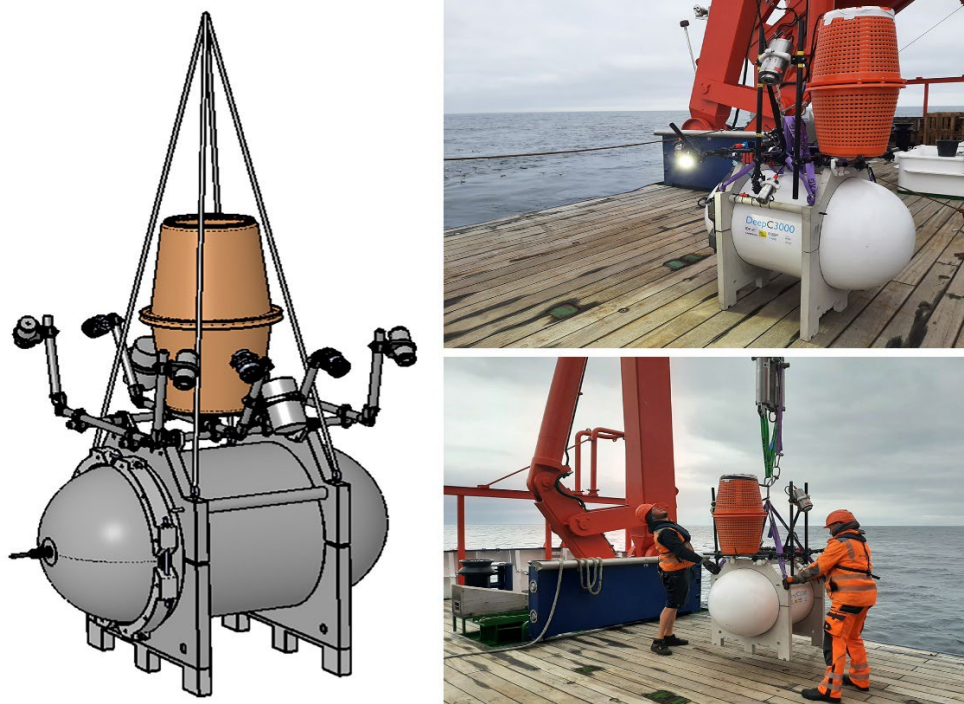
Fig. 5.6.2 The novel concrete-cylinder battery-system mooring with time-lapse cameras and lights attached. Left: Visualization showing the pressure housing made from carbon-reinforced concrete with mounts for cameras and flashes (in grey). Right: The system is deployed on 27 th of June 2022 on board RV MARIA S. MERIAN. The orange container on top holds 300 m mooring line released upon recovery (Visualization: F. Wenzhöfer et al., unpubl.; photographs: F. Janssen).
