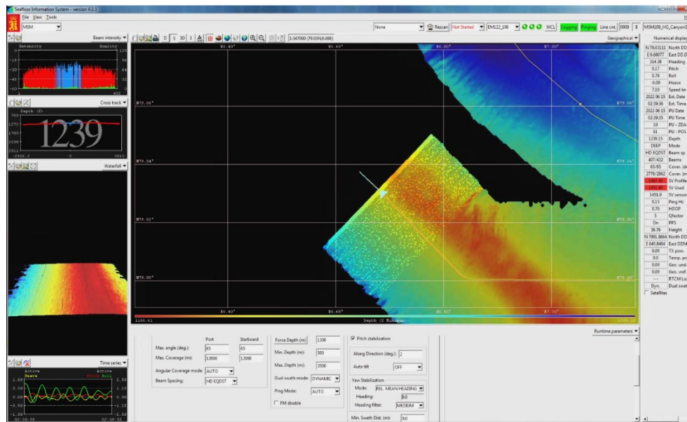
Fig. 5.4.1 Live view of the EM122 echosounder data collection during MSM108. The circular features on the red ridge toward the southeast are the array of pockmarks discovered during MSM108 (Photo: A. Purser).
