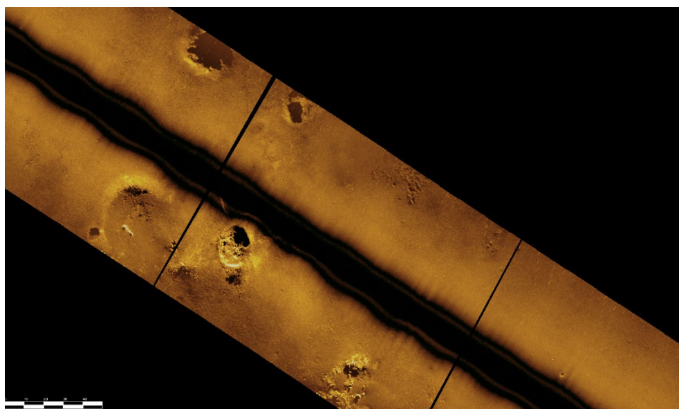
Fig. 5.4.3 Georeferenced acoustic data collected by the AUV ‘Paul’ and featuring several circular pockmarks.
