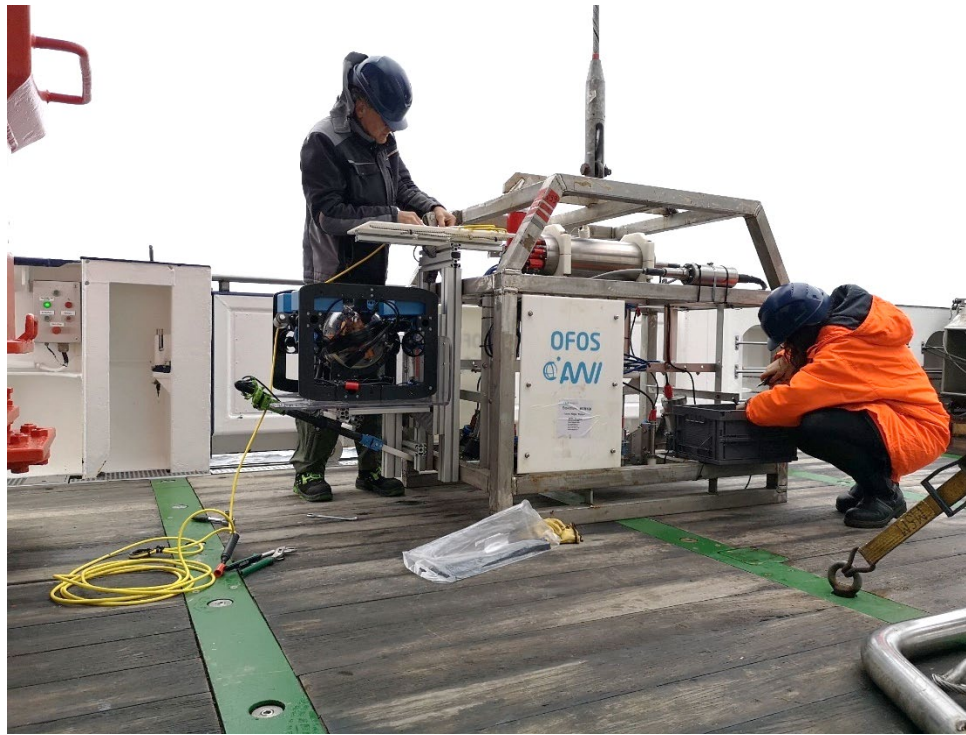
Fig. 5.2.4 The OFOS being prepared for operations during MSM108. The small ‘Remora’ class ROV is visible on the left of the frame (Photo: J. Schnier).
