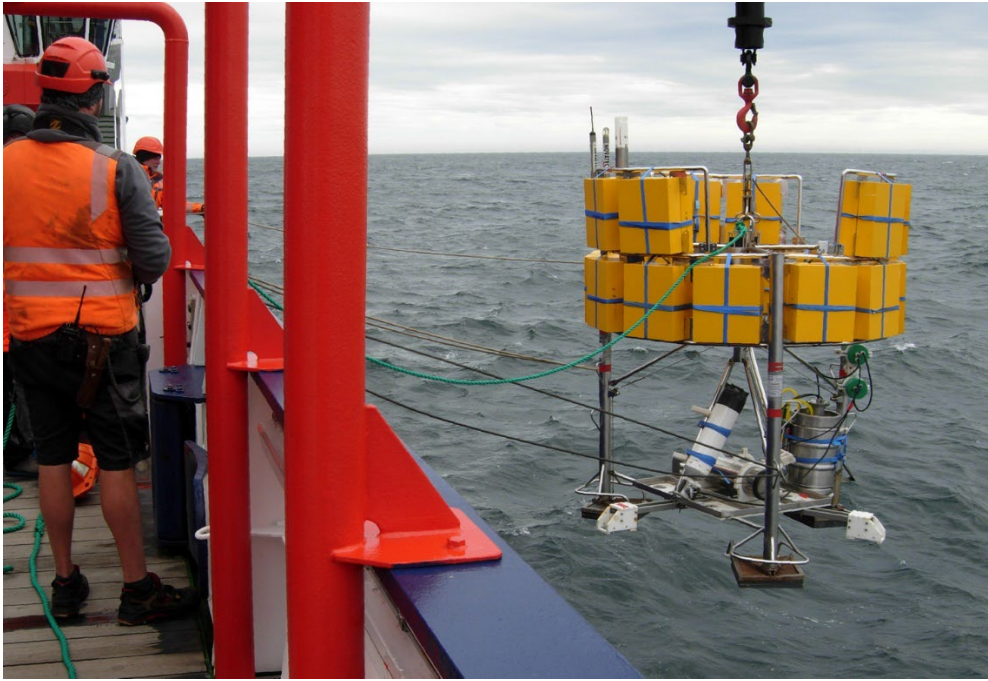
Fig. 5.7.1 Deployment of the Bottom-Lander based arcFOCE experimental set-up during expedition MSM108.
