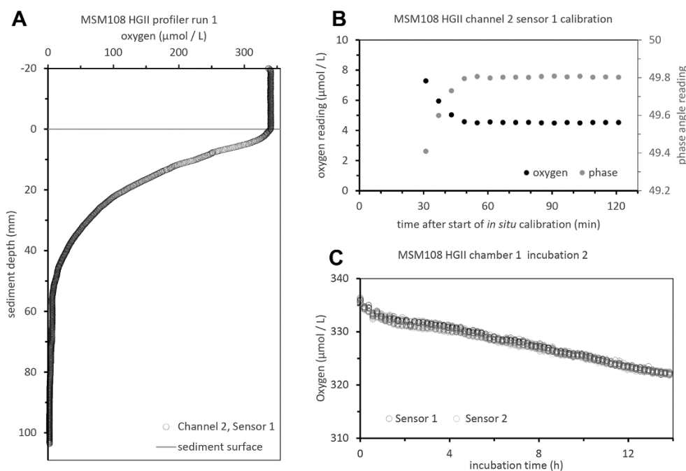
Fig. 5.6.4 Some preliminary plots of data collected with the crawler during the short deployment at station HG-II. Panel A: porewater oxygen profile recorded with a fiberoptical microsensor in the upper 10 cm of sediment. The grey line indicates the sediment surface. Panel B: sensor readings (oxygen and fluorescence phase angle) of the same fiberoptical sensor obtained after recording the profile shown in panel A while the sensor tip was flushed with oxygen-free calibration solution. The calibration information is used to correct microprofile raw oxygen data. Panel C: Time-series recording of oxygen concentrations in the overlying water of benthic chamber 1 during the second incubation. All oxygen data have been normalized to an estimated true bottom-water oxygen concentration of 335 \mu\text{mol L}^{-1} (F. Janssen, F. Wenzhöfer et al., unpublished data).
