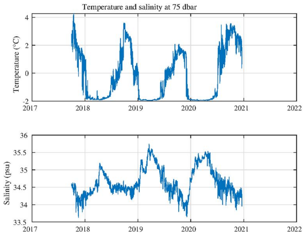
Figure 4. Temperature and salinity record at 75dbar from the mooring.
