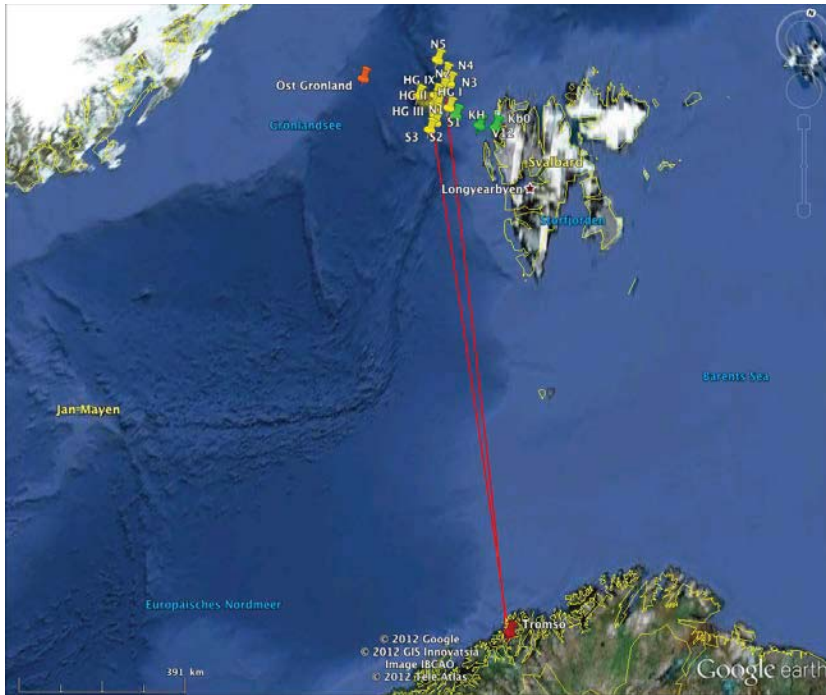
Fig. 1: Geographical area of the working area and transit route
