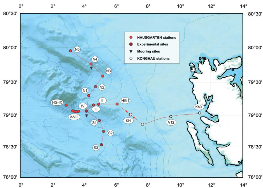
Fig. 2: Close-up of sampling sites for the HAUSGARTEN and Kongsfjord study area
