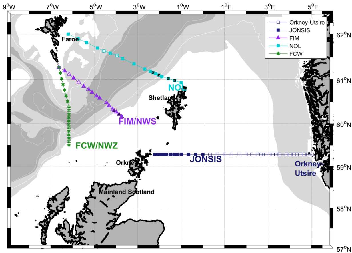
1919S: Hydrographic survey lines
