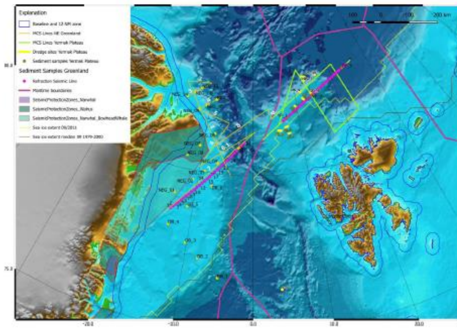
Fig. 2: Planned survey lines and stations in the survey area. The final location of the deployments will depend on the sea ice conditions.
