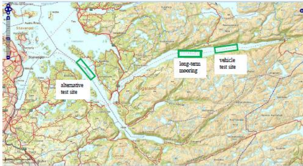
Fig. 3. Proposed model vehicle test area in Lysefjord, alternative test site in Høgsfjord, and site for deployment of long-term current meter mooring.
