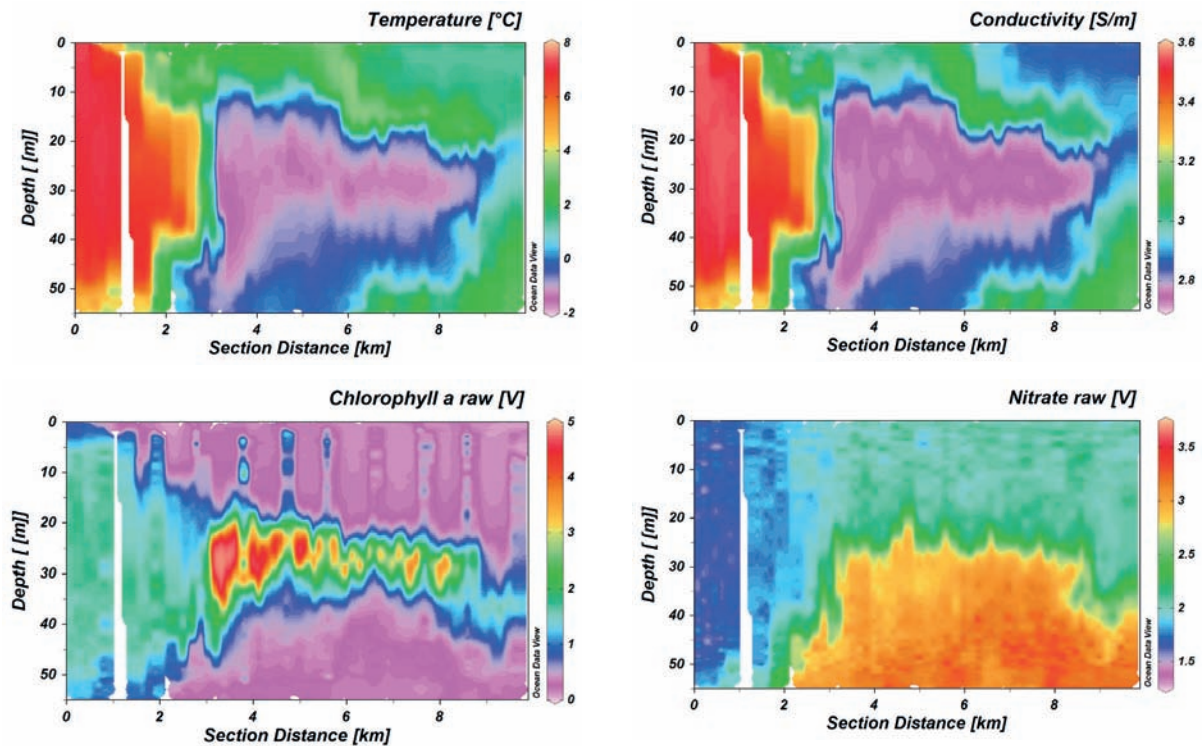
Fig. 7.4: (Upper left) temperature, (Upper right) conductivity, (Lower left) chlorophyll a, and (Lower right) nitrate data of PAUL's fourth dive
