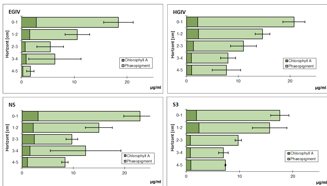
Fig. 11.2.2: Chloroplatic pigments in the upper five sediment centimetres at four selected stations at ~2,500 m water depth
