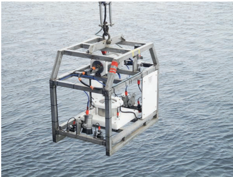
Fig. 11.4.1: The Ocean Floor Observation System (OFOS)
