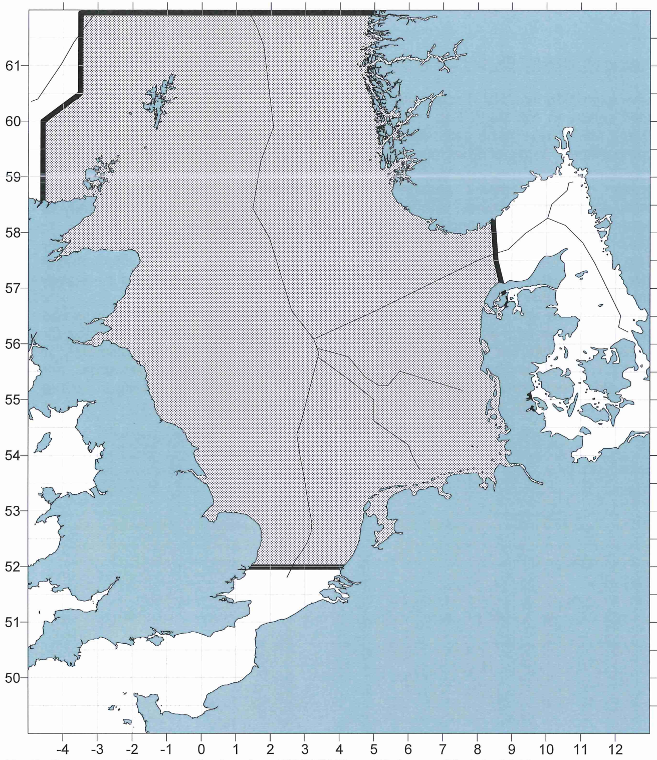
North Sea acoustic survey for herring, TRIDENS 27 June - 22 July 2016 The outer border of the survey area is indicated in black.
