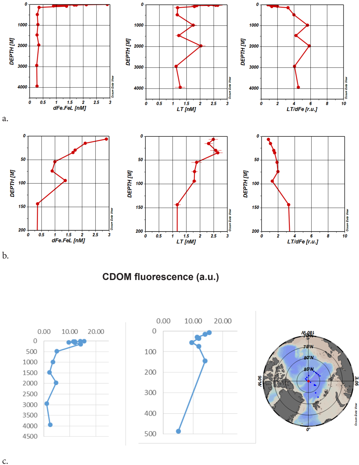
Fig. 6.5.1: Dissolved iron measured from ligand sample bottles ( dFe.FeL ), total ligand concentration ( LT ) and the ratio of LT and dFe for the entire depth profile (a) and for the upper 200 m (b). CDOM fluorescence for the entire depth profile and the upper 500 m (c).
