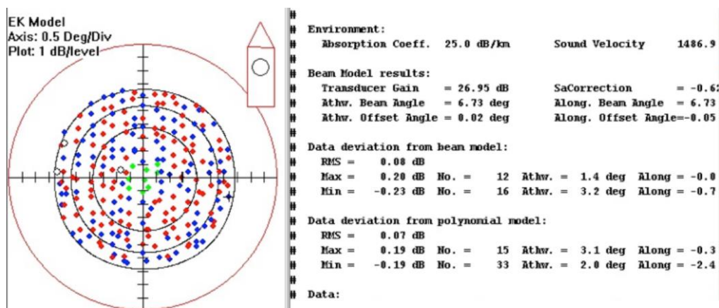
Figure 11: An example of a good EK60 calibration model. All points are located within 3 dB range. Green dots show target locations near the main acoustic center of the echo sounder. Red and blue dots show data, whose target strengths are larger or smaller in comparison to the model results. Very good calibration outcomes result in (i) symmetric distribution of targets within beam and (ii) random distributions of red and blue dots, and as a result a small deviation from the beam model (RMS < 0.1 dB).
