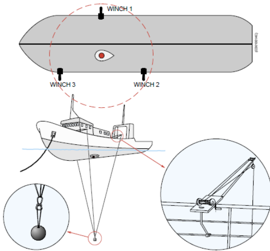
Figure 4: Schematic drawing of lowering the copper sphere into the sound beam.
