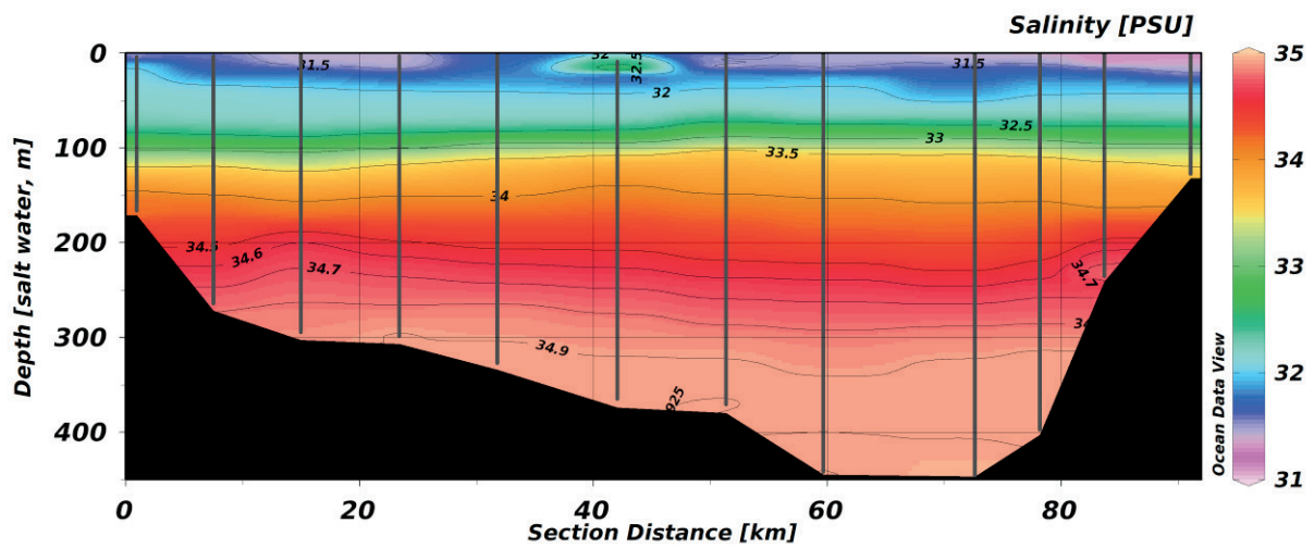
Fig. 5.4: Salinity from CTD casts along the Norske Trough section. Locations of CTD casts are denoted by thick grey lines.
