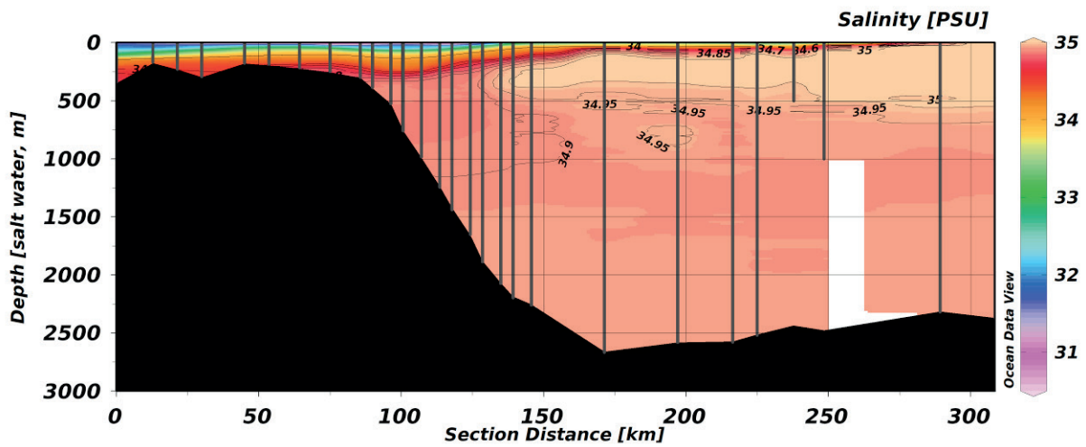
Fig. 5.7: Salinity from CTD casts along the section at 78° 50' N: full-depth. Locations of CTD casts are denoted by thick grey lines
