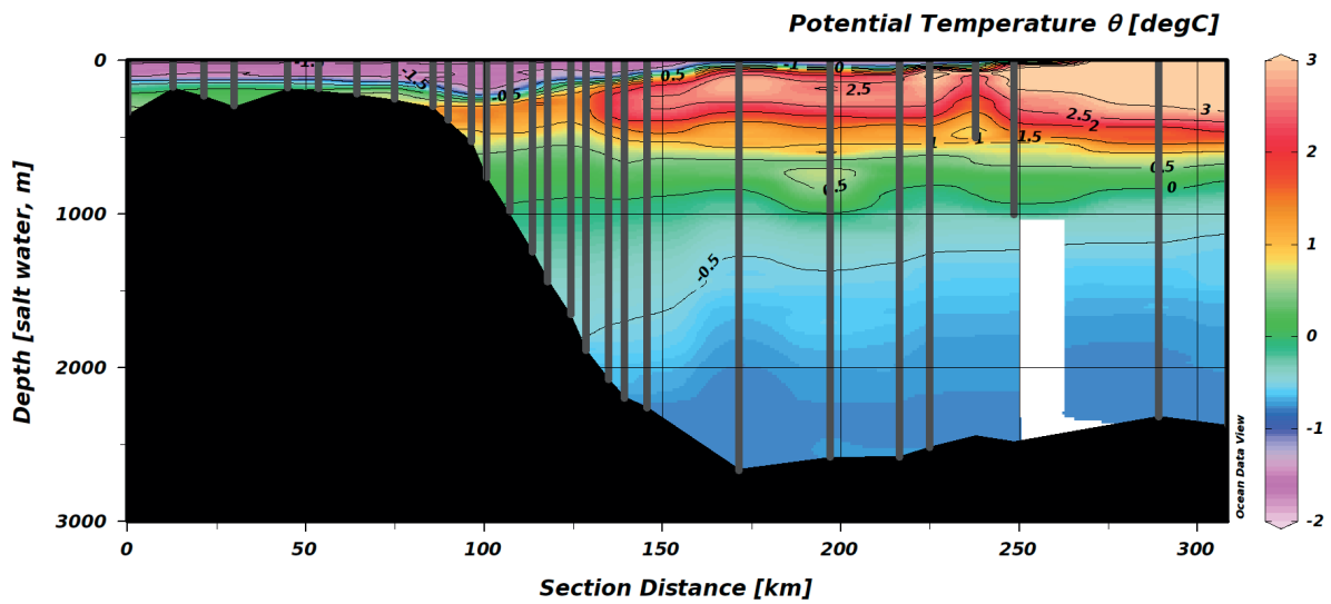
Fig. 5.5: Potential temperature from CTD casts along the section at 78° 50' N: full-depth. Locations of CTD casts are denoted by thick grey lines.
