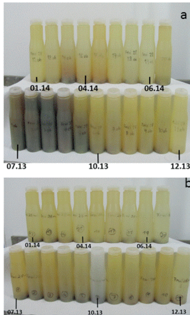
Fig. 8.4: Sampling jars of an annually moored sediment trap at Station HGIV from 07/2013 till 06/2014; samples from the trap moored at ~200 m below the surface (a) and from ~1,100 m (b).
