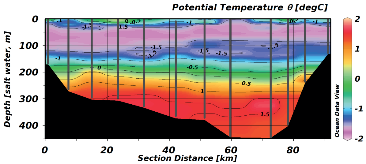
Fig. 5.3: Potential temperature, referenced to 0 dbar, from CTD casts along the Norske Trough section. Locations of CTD casts are denoted by thick grey lines.
