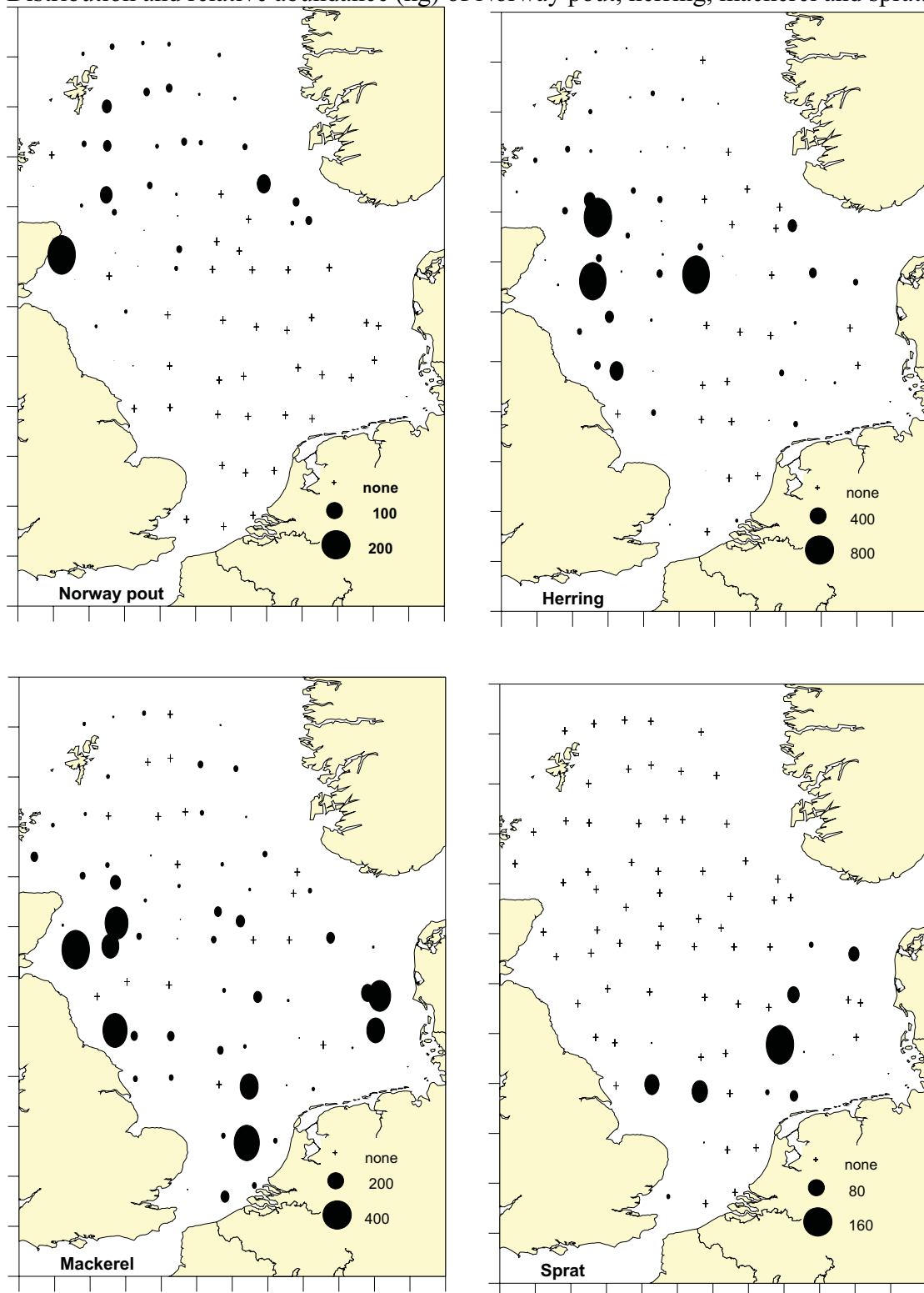
Figure 3. Distribution and relative abundance (kg) of Norway pout, herring, mackerel and sprat.
