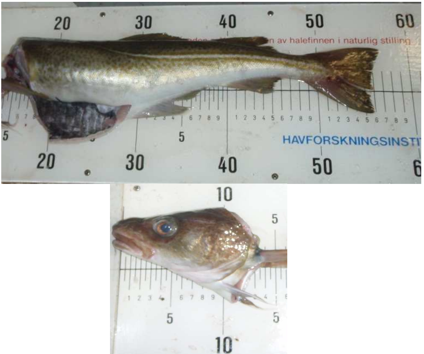
Fig.3.1.4. Photo of the product gutted cod without head and earbones, processed by machine.
